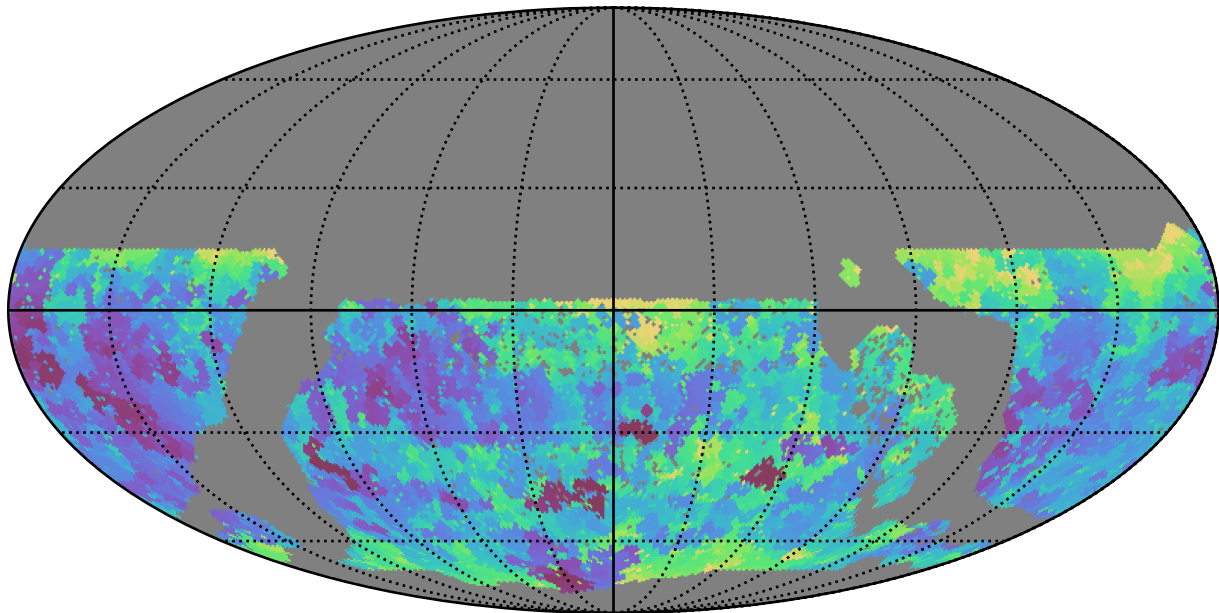
too_elab_r128_d2_griz_v3.4_10yrs WFD u band: Min seeingEff
