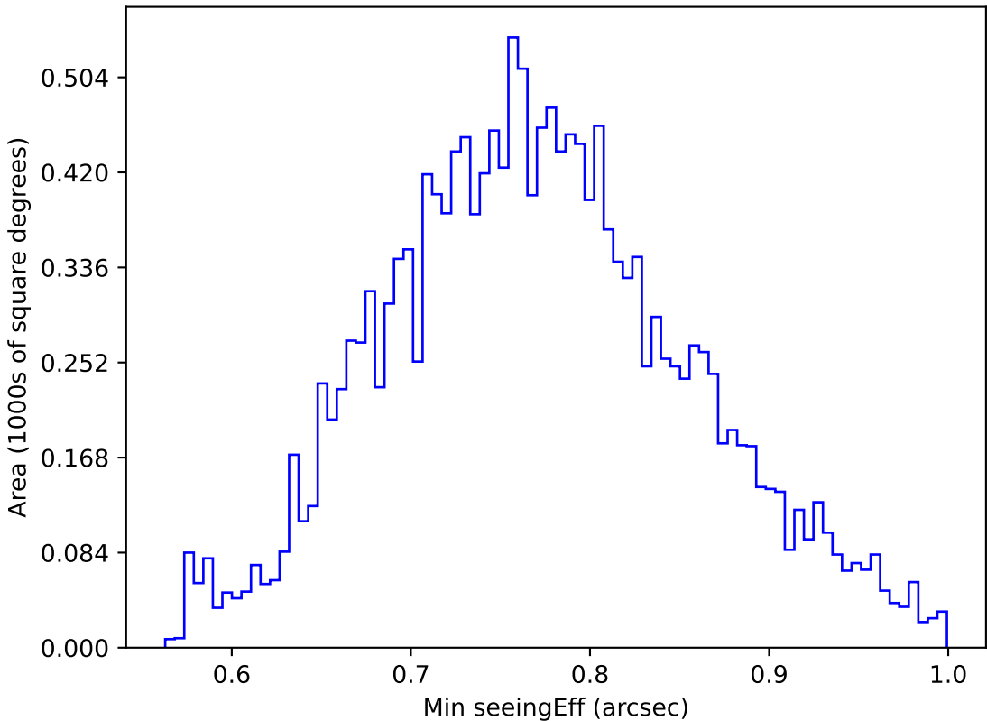
too_elab_r128_d2_griz_v3.4_10yrs WFD u band: Min seeingEff
