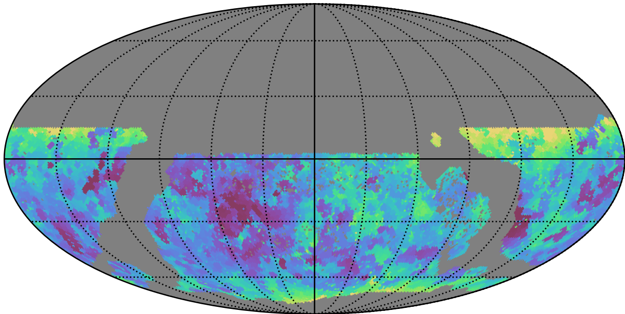
too_elab_r128_d2_griz_v3.4_10yrs WFD r band: Min seeingEff
