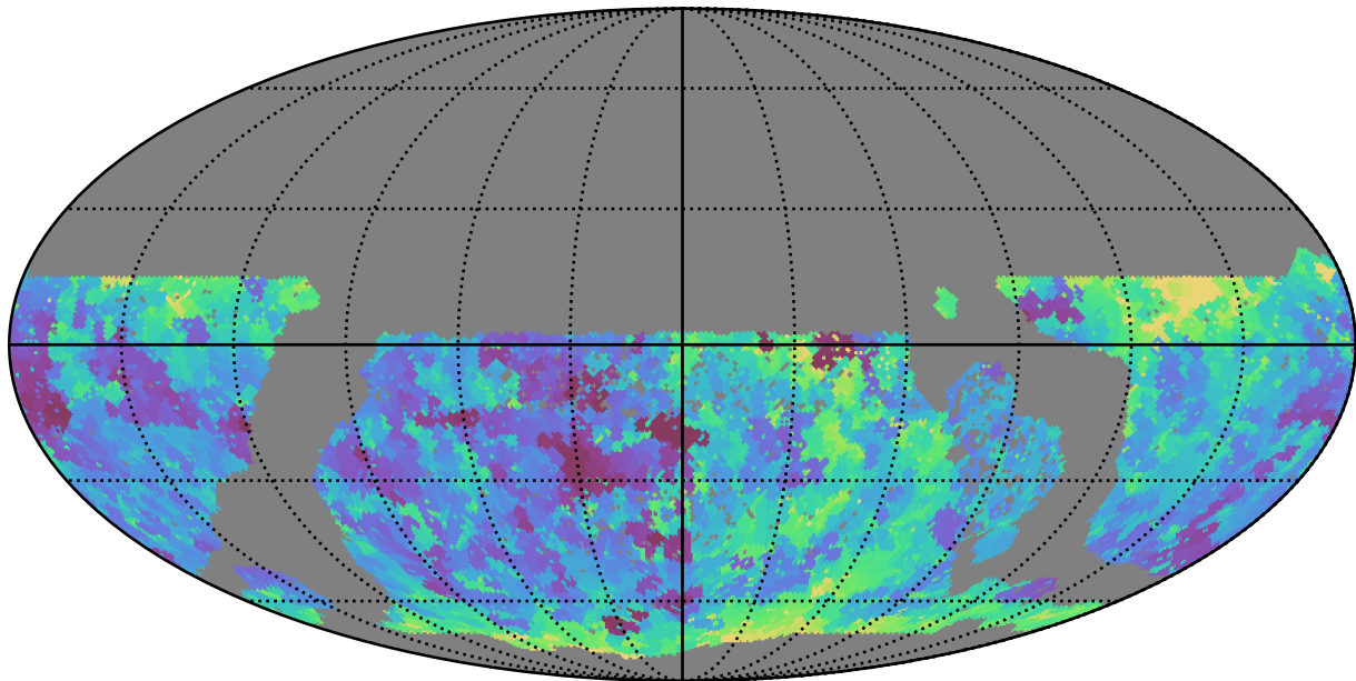
too_elab_r128_d2_griz_v3.4_10yrs WFD g band: Min seeingEff
