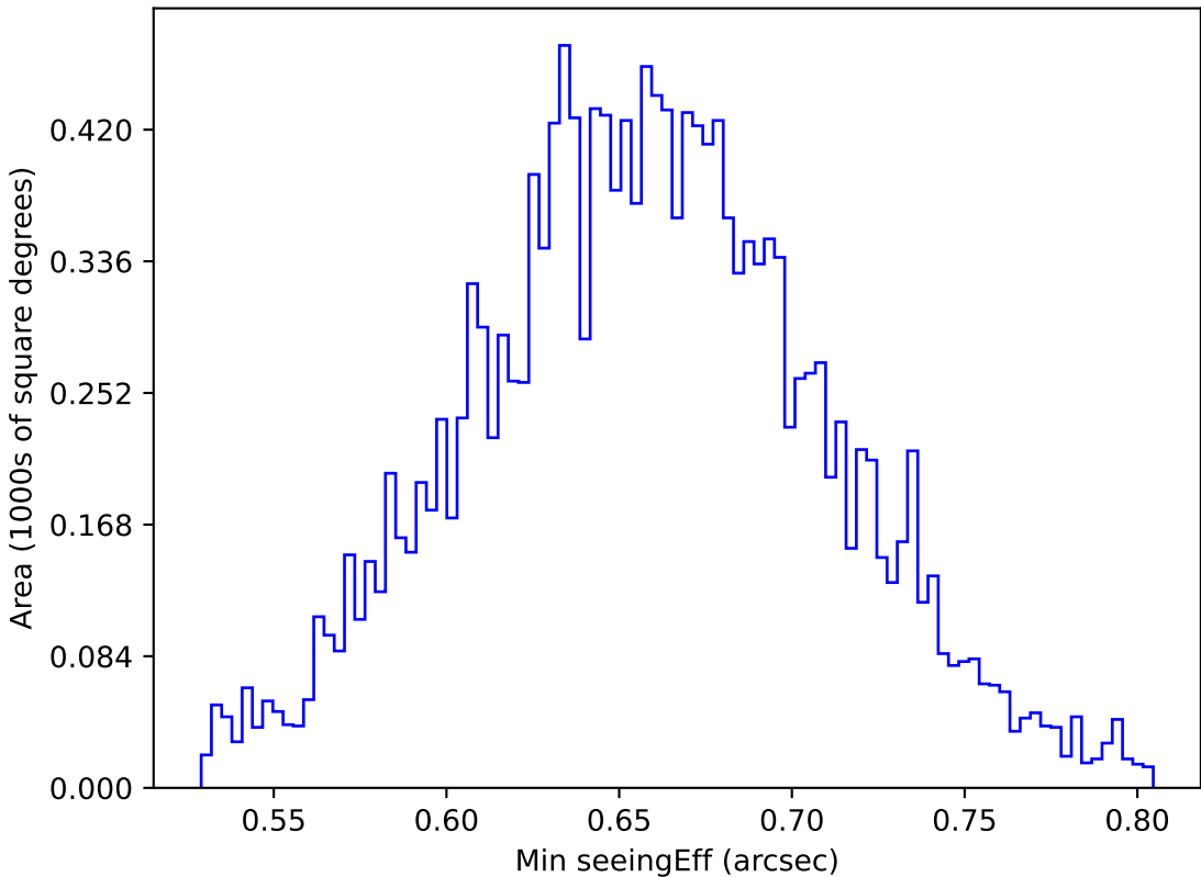
too_elab_r128_d2_griz_v3.4_10yrs WFD g band: Min seeingEff
