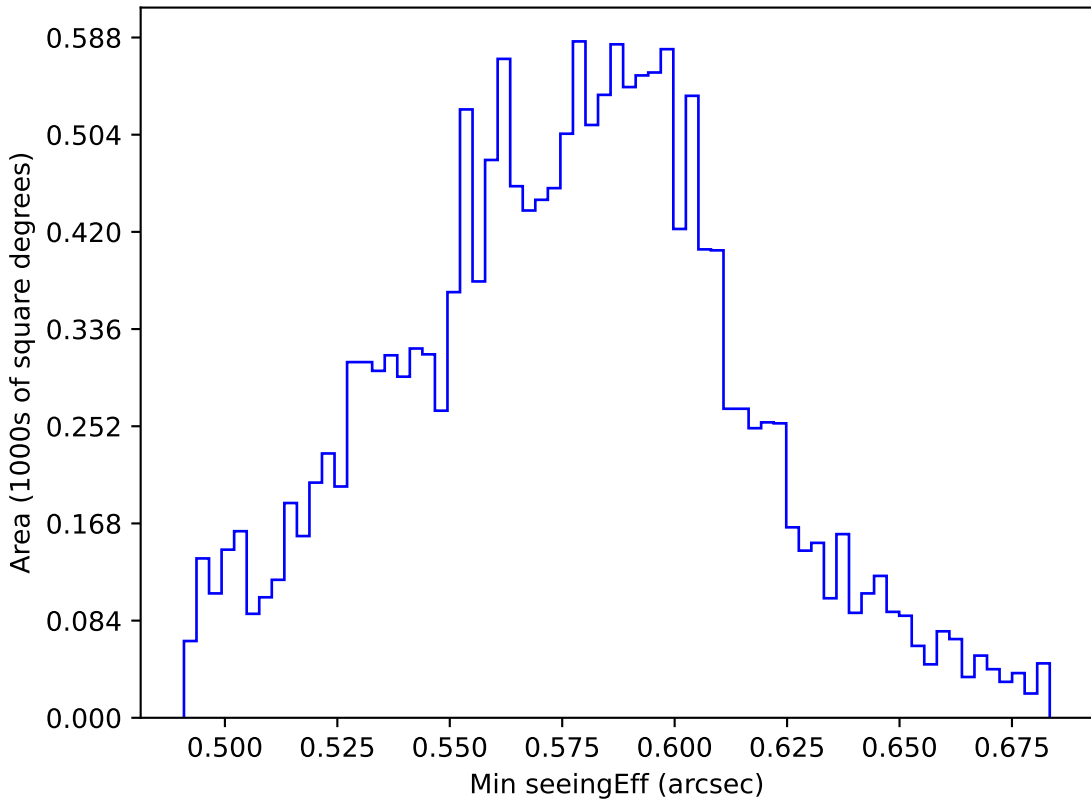
too_elab_r128_d2_griz_v3.4_10yrs WFD all bands: Min seeingEff
