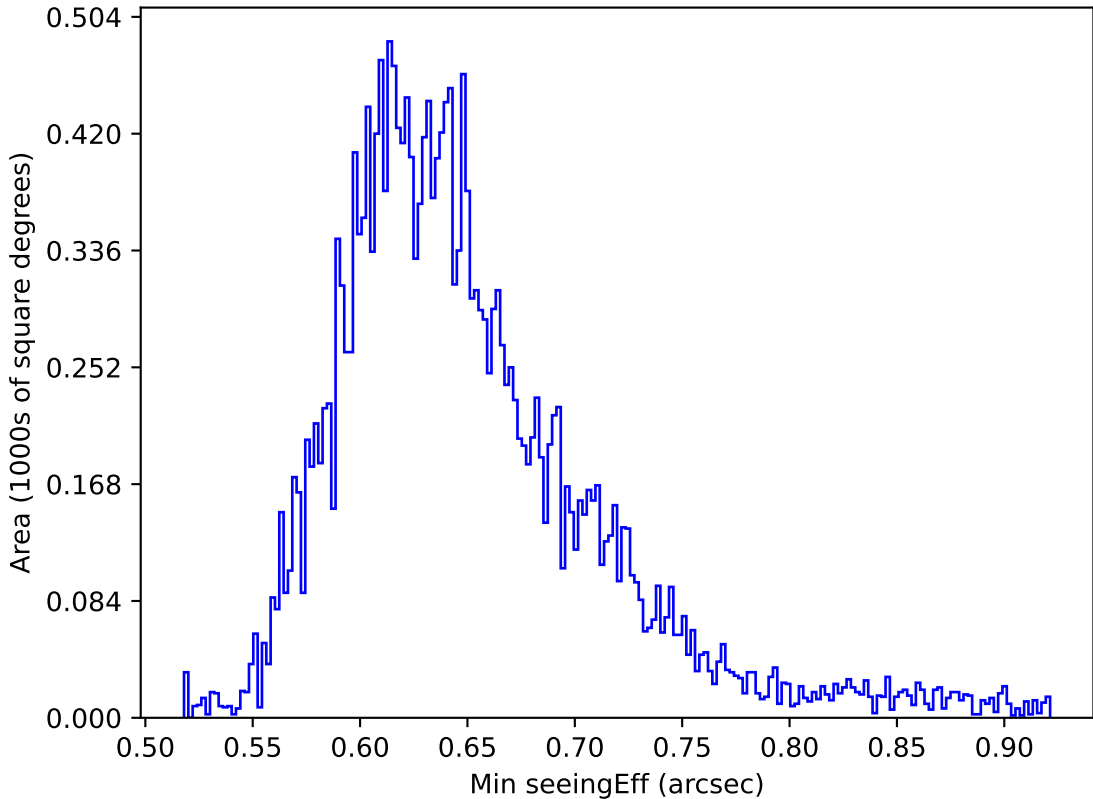
too_elab_r128_d2_griz_v3.4_10yrs All sky y band: Min seeingEff
