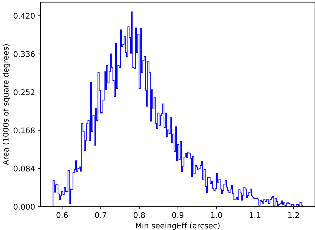
too_elab_r128_d2_griz_v3.4_10yrs All sky u band: Min seeingEff
