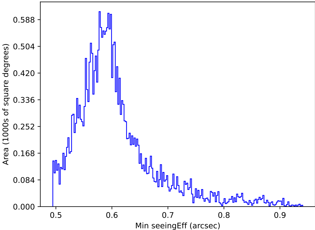
too_elab_r128_d2_griz_v3.4_10yrs All sky all bands: Min seeingEff
