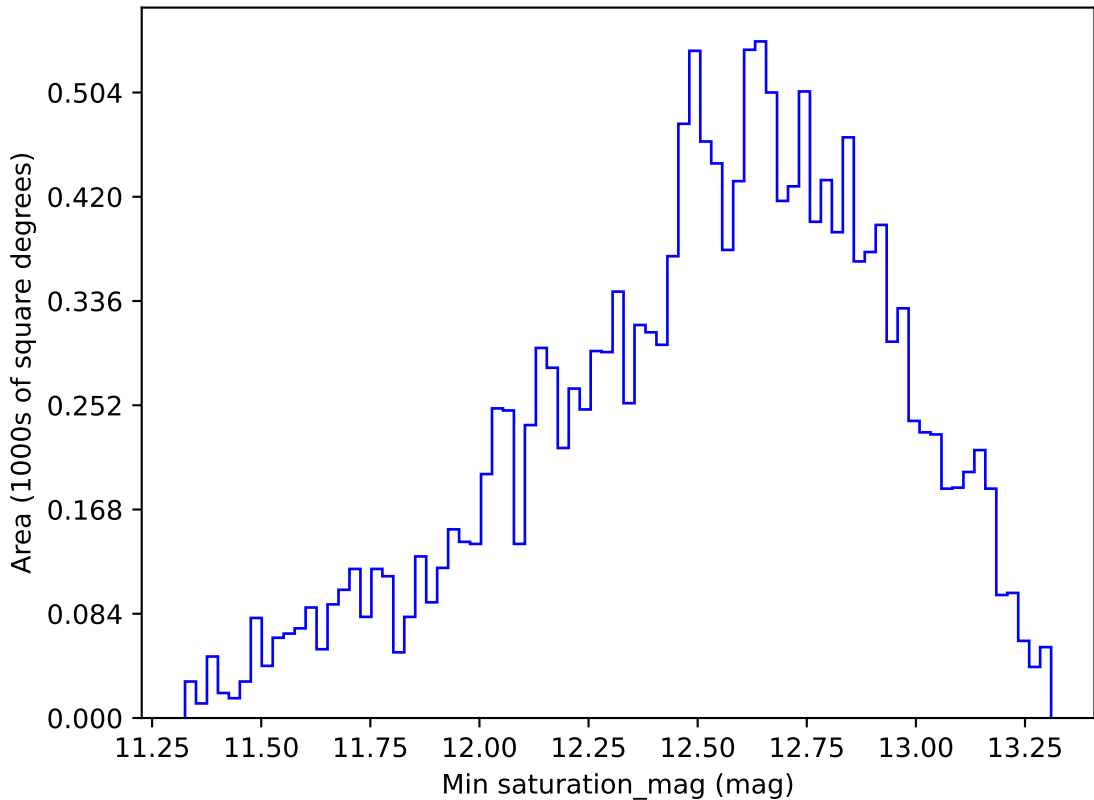
too_elab_r128_d2_griz_v3.4_10yrs WFD r band: Min saturation_mag
