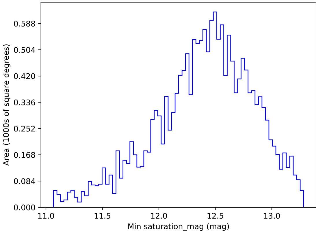
too_elab_r128_d2_griz_v3.4_10yrs WFD i band: Min saturation_mag
