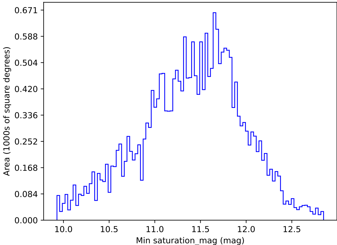
too_elab_r128_d2_griz_v3.4_10yrs All sky u band: Min saturation_mag
