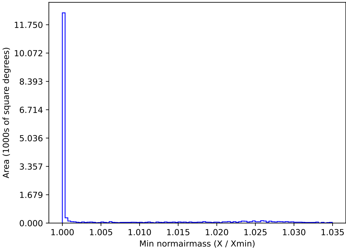
too_elab_r128_d2_griz_v3.4_10yrs WFD z band: Min normairmass
