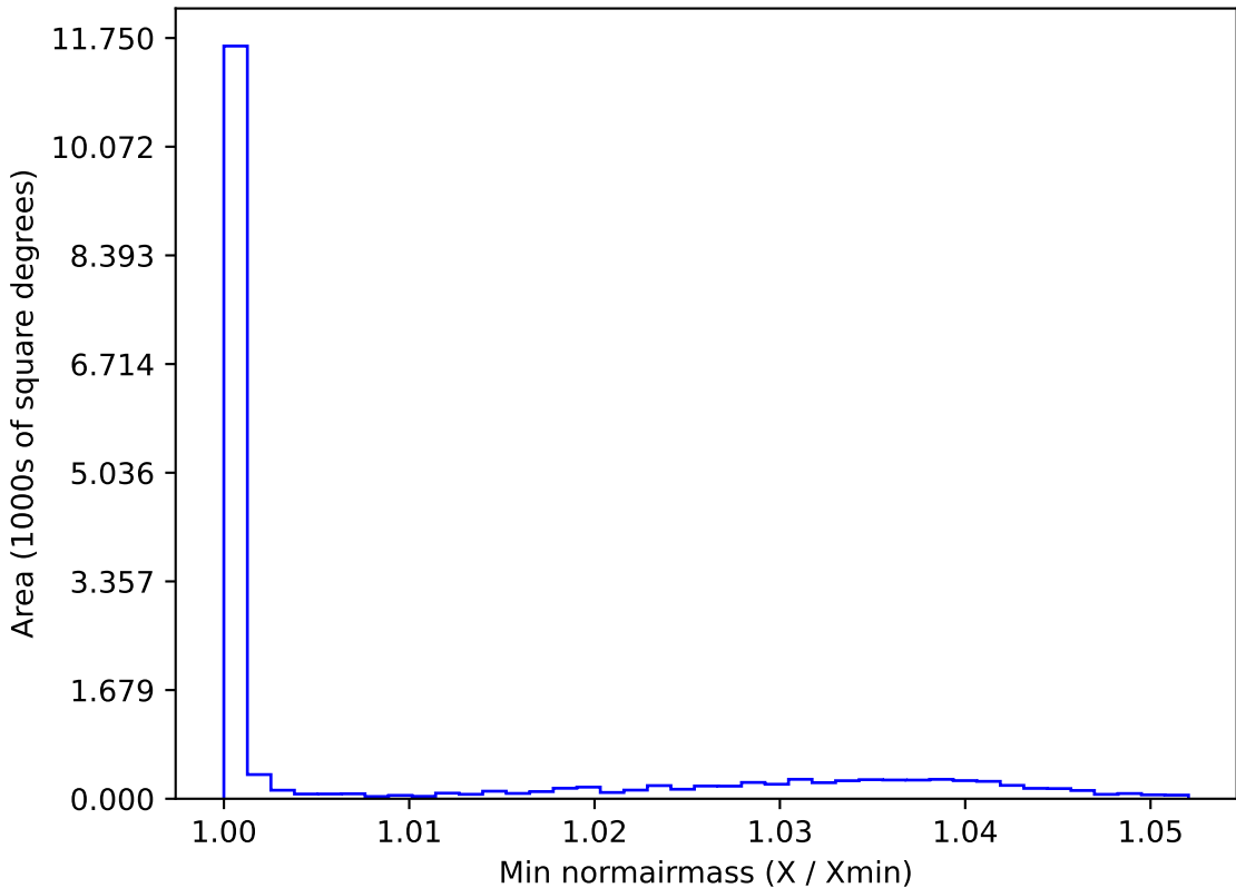
too_elab_r128_d2_griz_v3.4_10yrs WFD u band: Min normairmass
