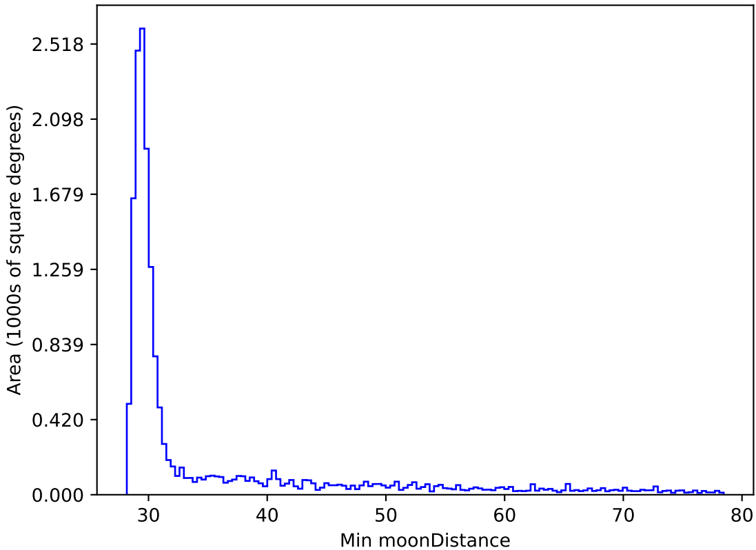
too_elab_r128_d2_griz_v3.4_10yrs WFD y band: Min moonDistance
