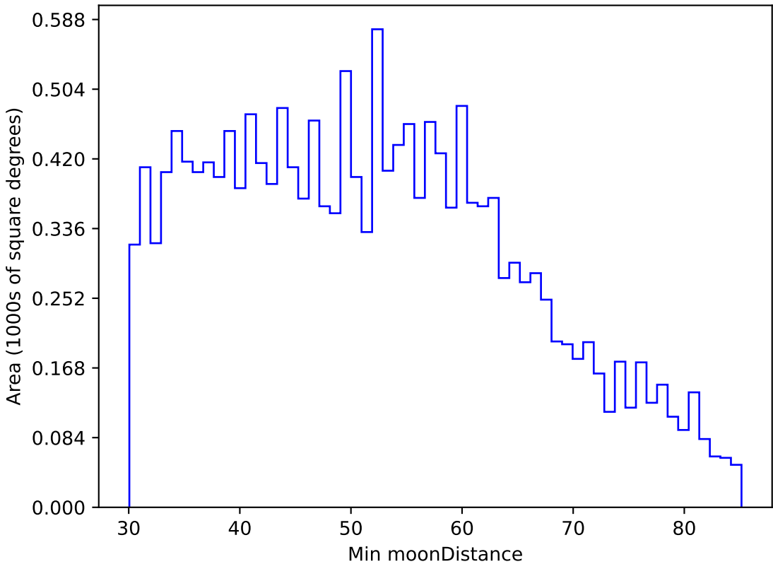
too_elab_r128_d2_griz_v3.4_10yrs WFD u band: Min moonDistance
