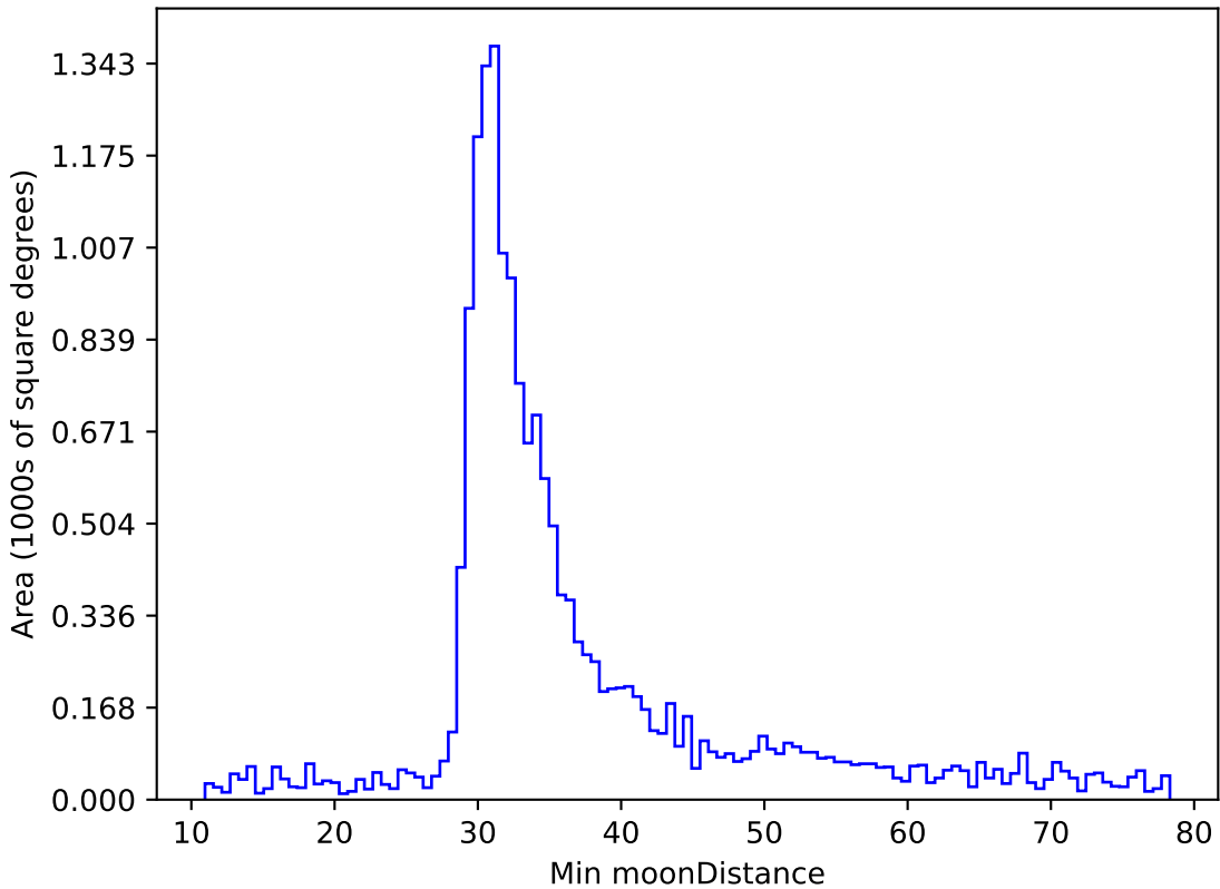
too_elab_r128_d2_griz_v3.4_10yrs WFD r band: Min moonDistance
