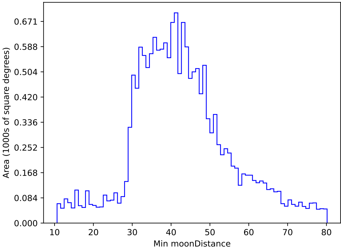
too_elab_r128_d2_griz_v3.4_10yrs WFD g band: Min moonDistance
