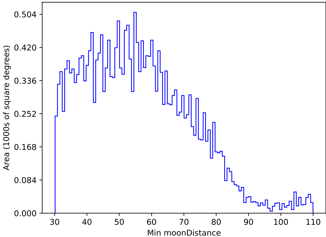
too_elab_r128_d2_griz_v3.4_10yrs All sky u band: Min moonDistance
