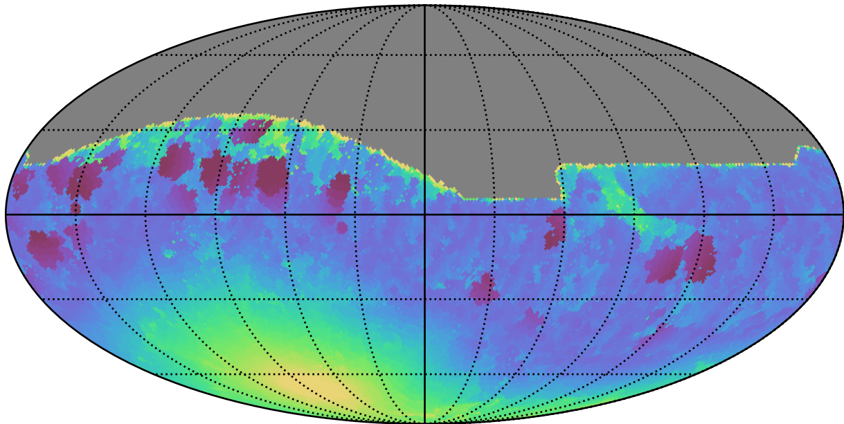
too_elab_r128_d2_griz_v3.4_10yrs All sky r band: Min moonDistance
