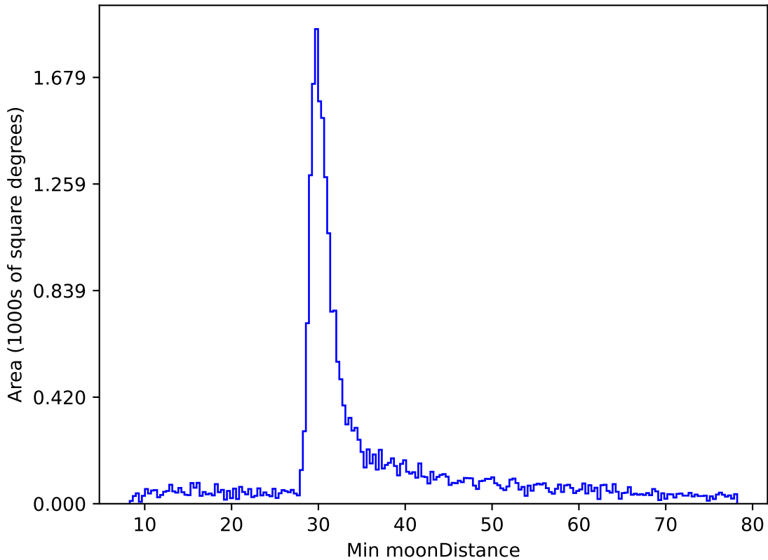
too_elab_r128_d2_griz_v3.4_10yrs All sky i band: Min moonDistance
