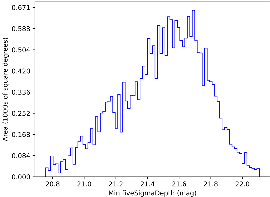
too_elab_r128_d2_griz_v3.4_10yrs Yr 1 y band: Min fiveSigmaDepth
