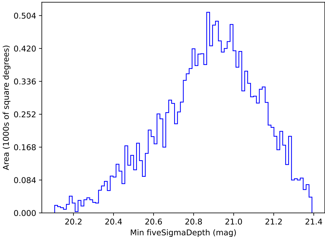
too_elab_r128_d2_griz_v3.4_10yrs WFD y band: Min fiveSigmaDepth
