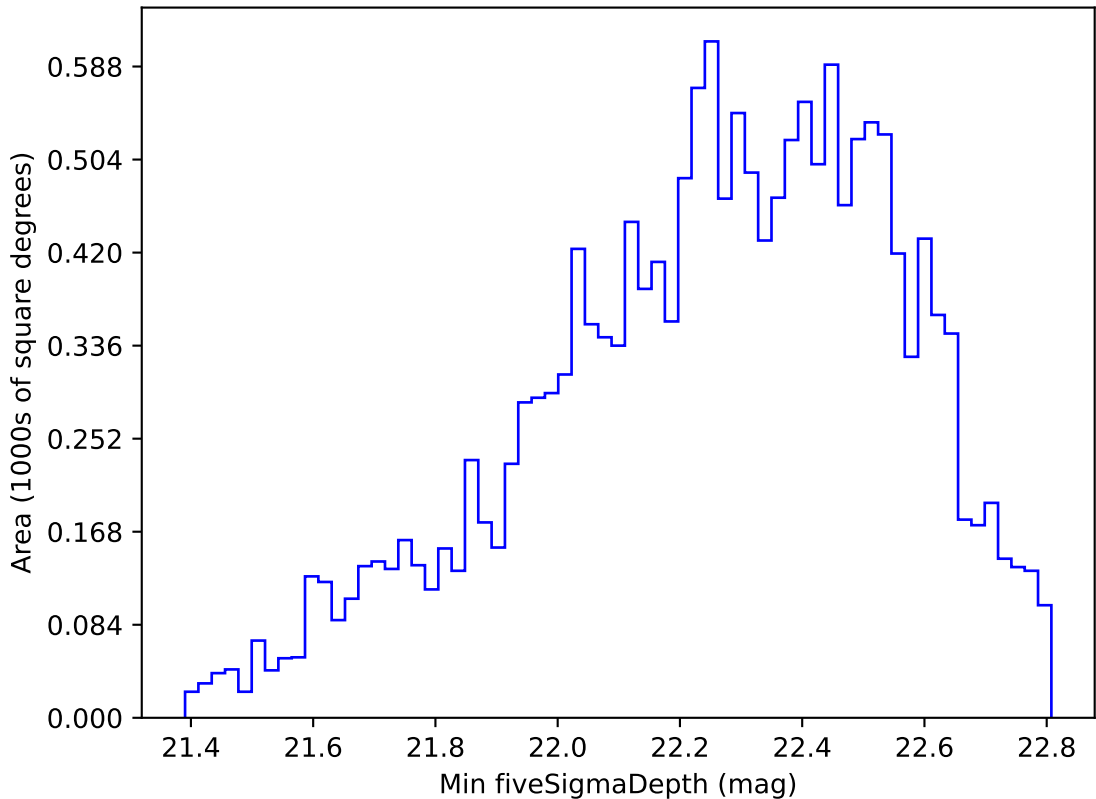
too_elab_r128_d2_griz_v3.4_10yrs WFD u band: Min fiveSigmaDepth
