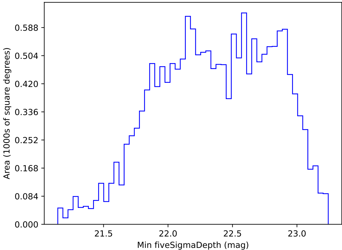
too_elab_r128_d2_griz_v3.4_10yrs WFD r band: Min fiveSigmaDepth
