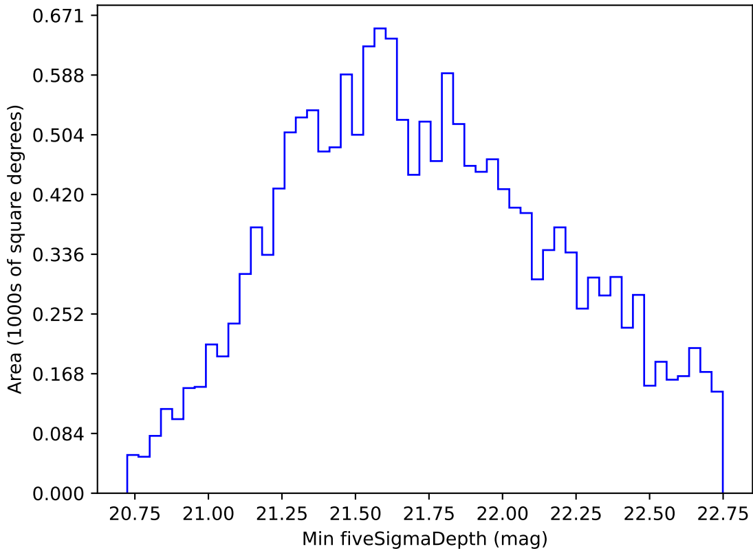
too_elab_r128_d2_griz_v3.4_10yrs WFD i band: Min fiveSigmaDepth
