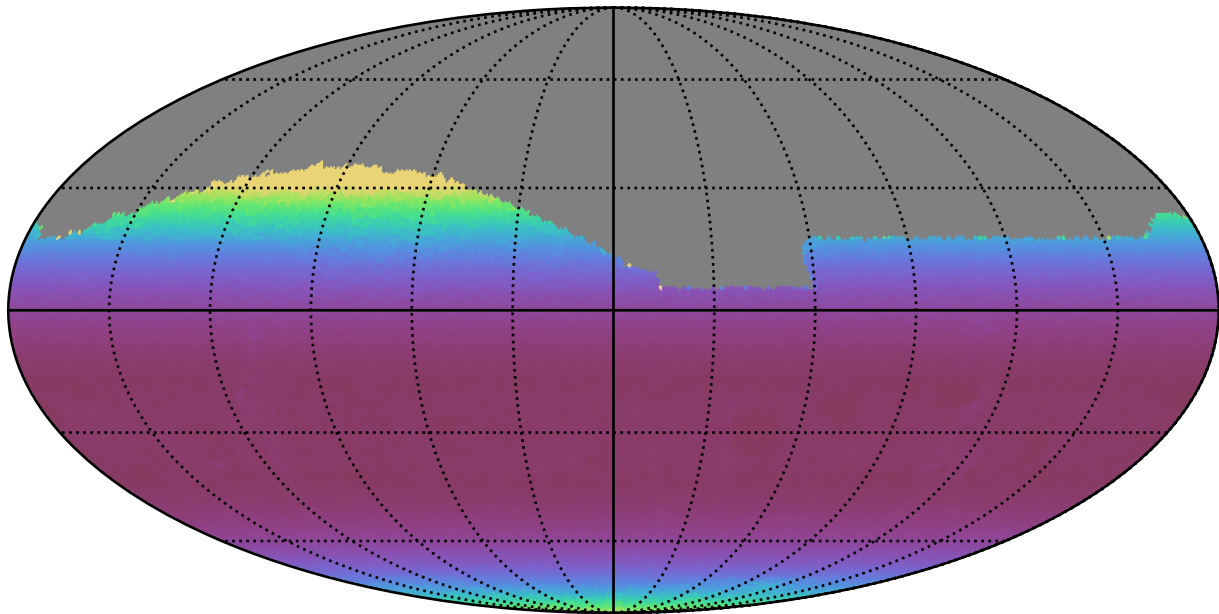
too_elab_r128_d2_griz_v3.4_10yrs Yr 1 all bands: Min airmass
