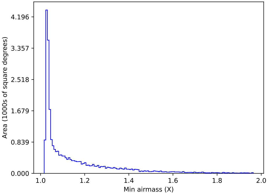
too_elab_r128_d2_griz_v3.4_10yrs Yr 1 all bands: Min airmass
