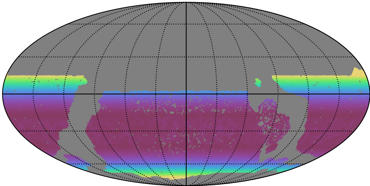
too_elab_r128_d2_griz_v3.4_10yrs WFD y band: Min airmass
