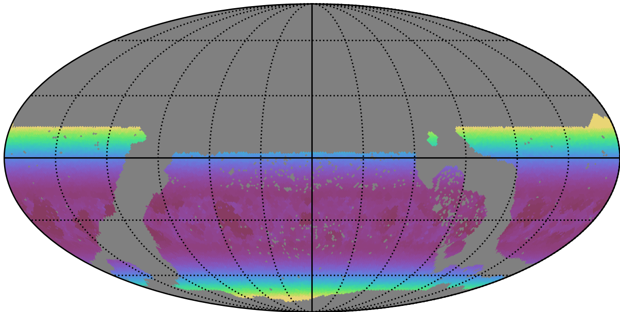
too_elab_r128_d2_griz_v3.4_10yrs WFD g band: Min airmass
