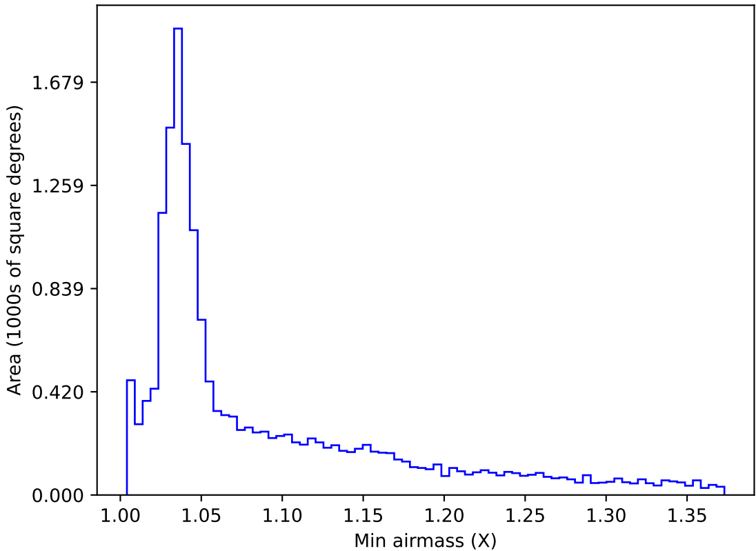
too_elab_r128_d2_griz_v3.4_10yrs WFD g band: Min airmass
