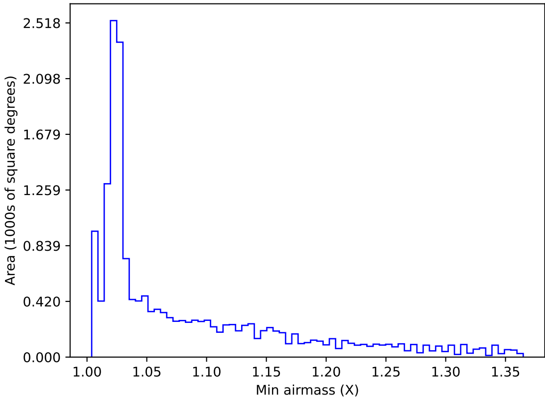
too_elab_r128_d2_griz_v3.4_10yrs WFD all bands: Min airmass
