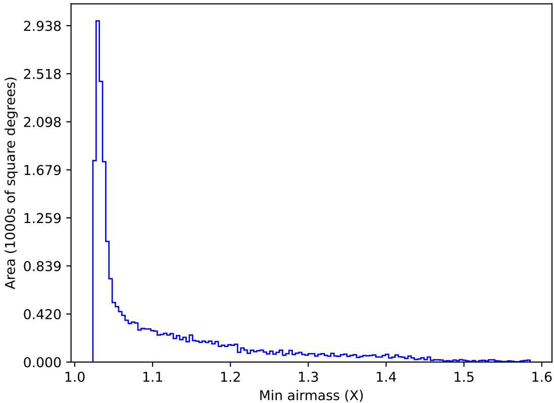
too_elab_r128_d2_griz_v3.4_10yrs All sky y band: Min airmass
