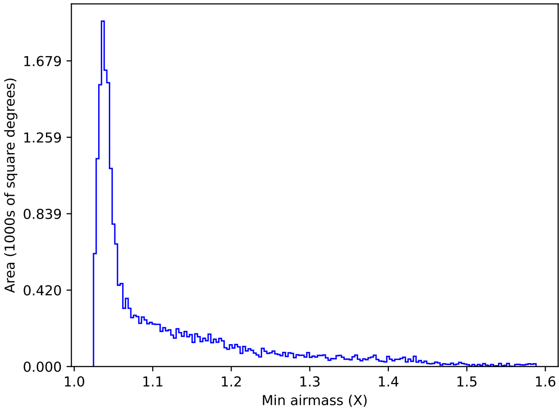
too_elab_r128_d2_griz_v3.4_10yrs All sky u band: Min airmass
