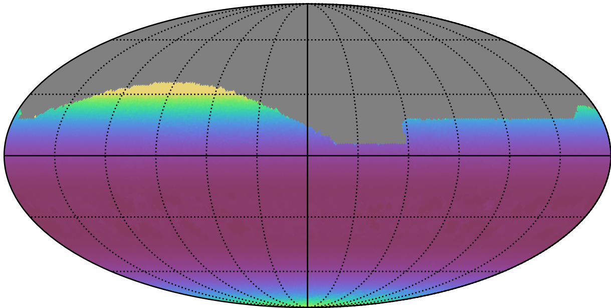
too_elab_r128_d2_griz_v3.4_10yrs All sky r band: Min airmass
