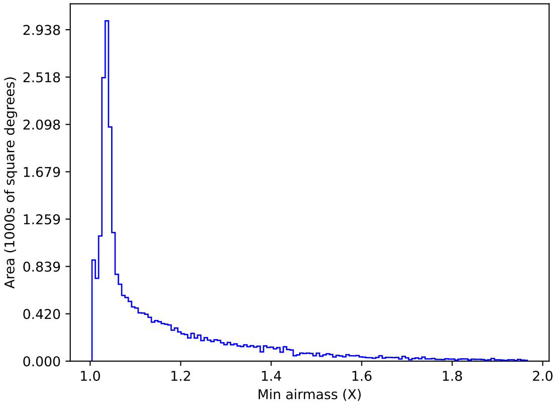
too_elab_r128_d2_griz_v3.4_10yrs All sky g band: Min airmass
