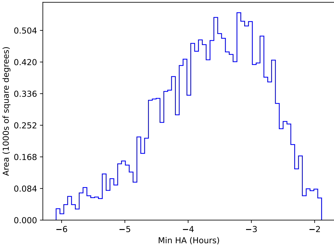
too_elab_r128_d2_griz_v3.4_10yrs WFD y band: Min HA
