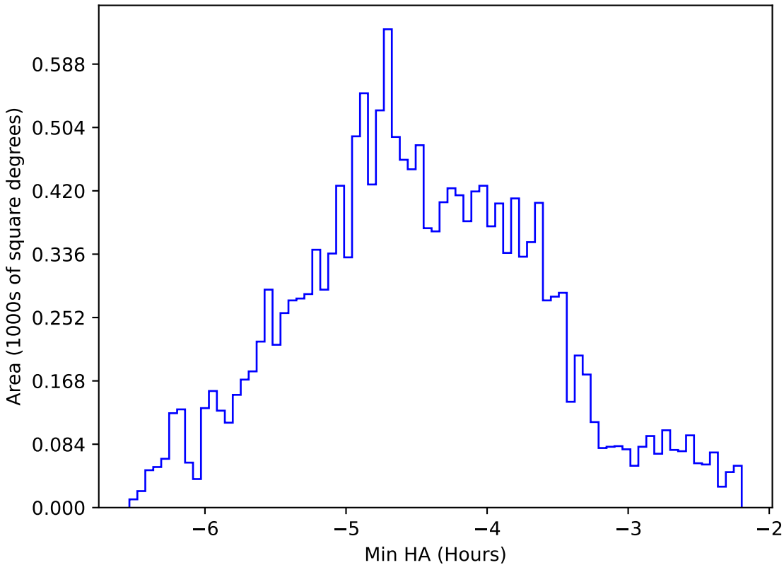
too_elab_r128_d2_griz_v3.4_10yrs WFD i band: Min HA
