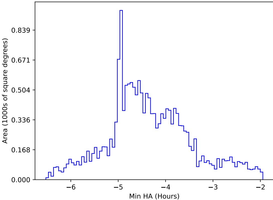
too_elab_r128_d2_griz_v3.4_10yrs WFD g band: Min HA
