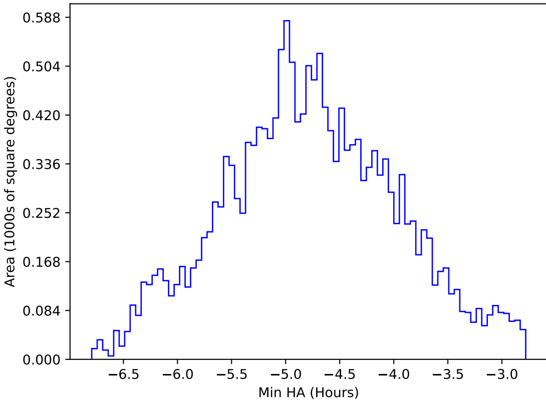
too_elab_r128_d2_griz_v3.4_10yrs WFD all bands: Min HA
