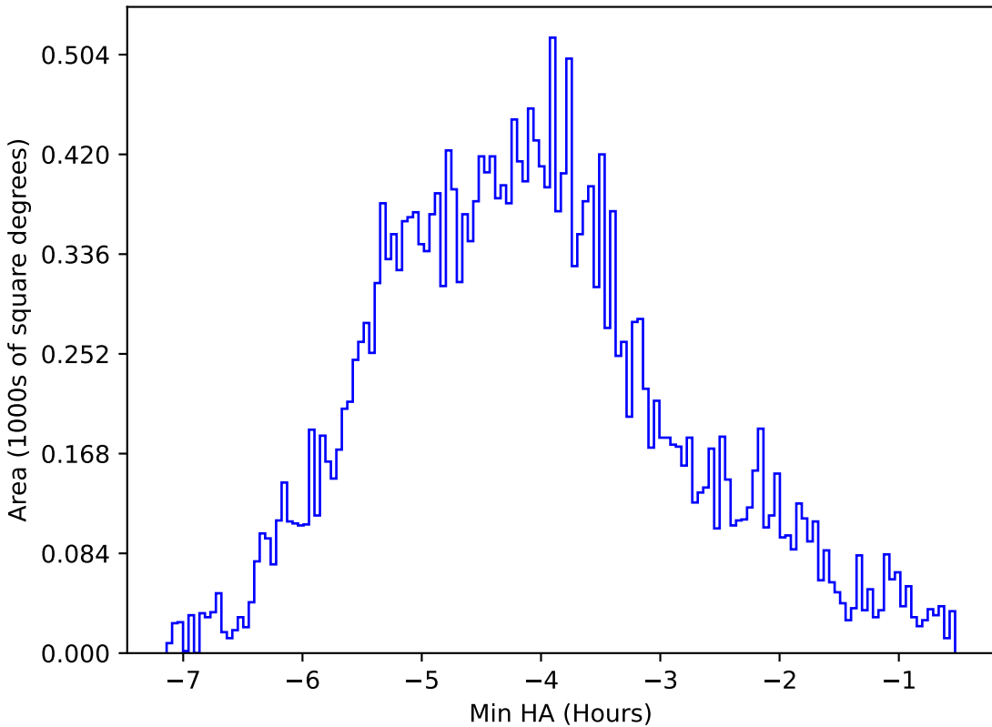
too_elab_r128_d2_griz_v3.4_10yrs All sky z band: Min HA
