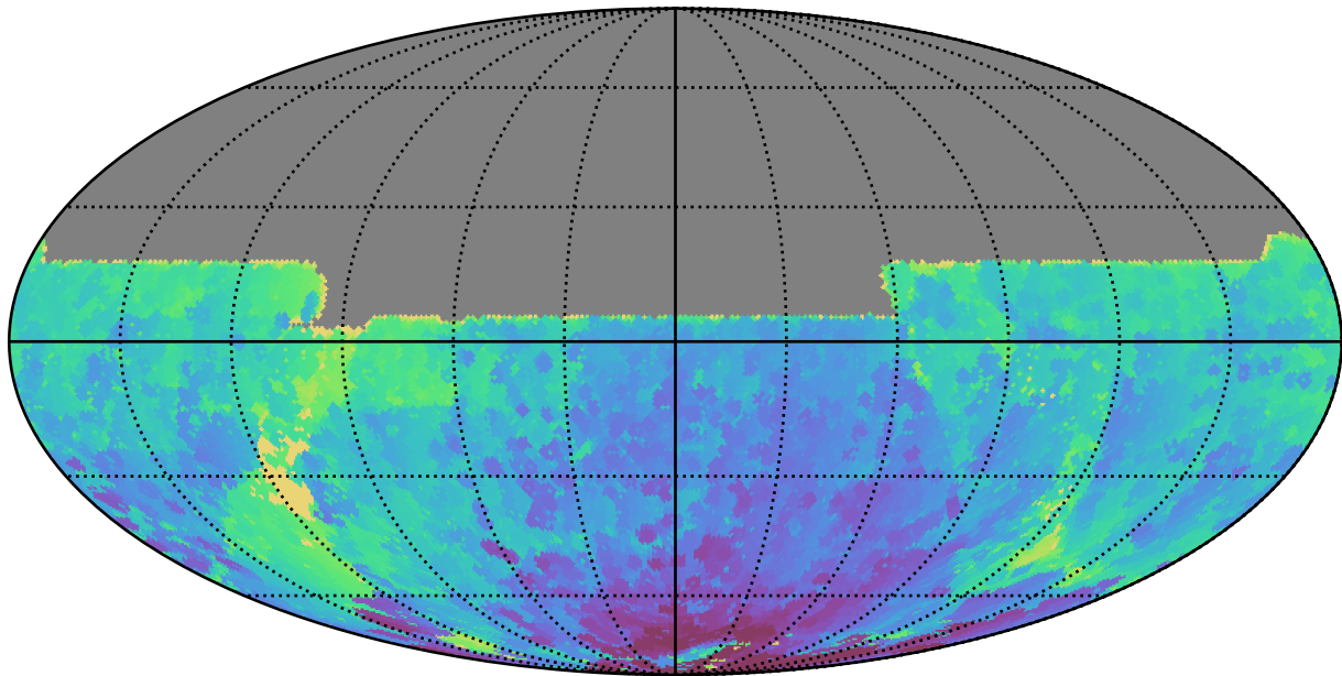
too_elab_r128_d2_griz_v3.4_10yrs All sky y band: Min HA
