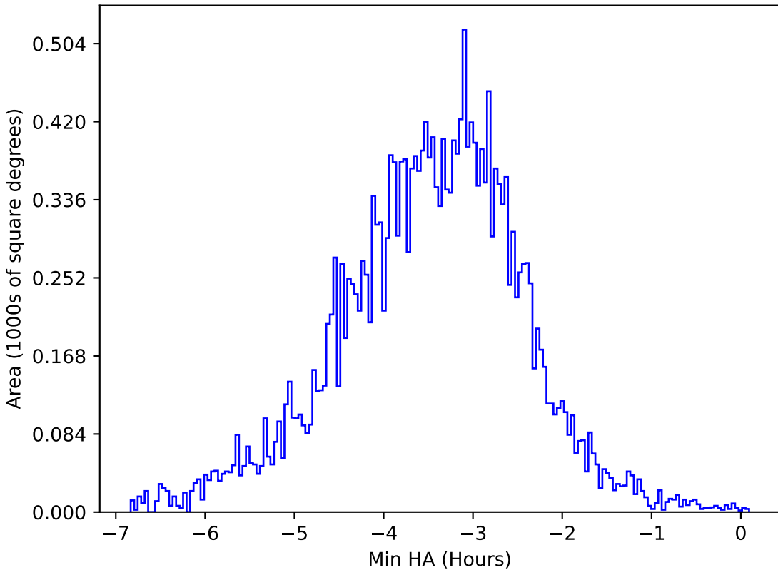
too_elab_r128_d2_griz_v3.4_10yrs All sky y band: Min HA
