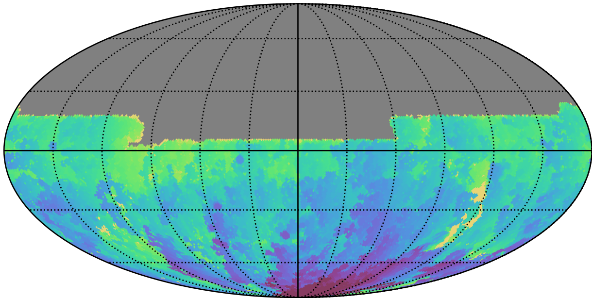
too_elab_r128_d2_griz_v3.4_10yrs All sky u band: Min HA
