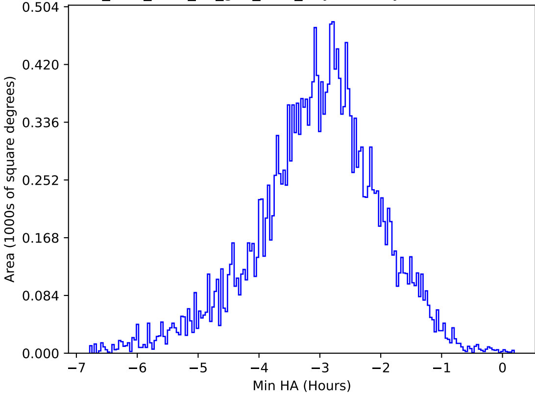
too_elab_r128_d2_griz_v3.4_10yrs All sky u band: Min HA
