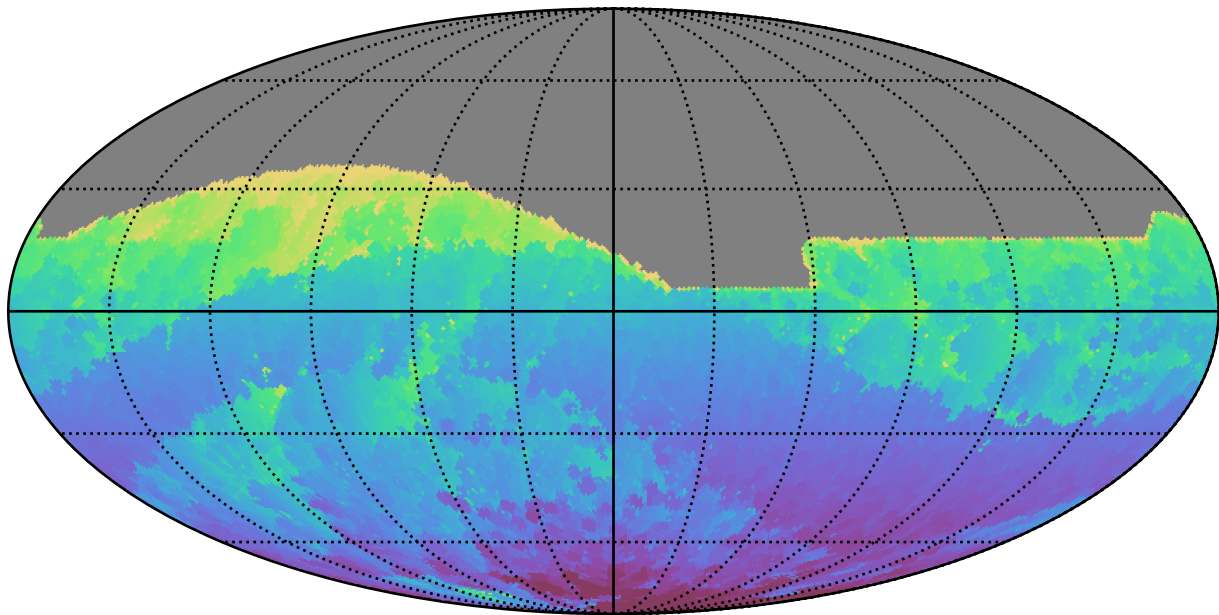
too_elab_r128_d2_griz_v3.4_10yrs All sky r band: Min HA
