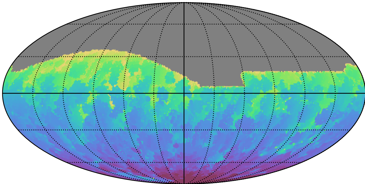
too_elab_r128_d2_griz_v3.4_10yrs All sky g band: Min HA
