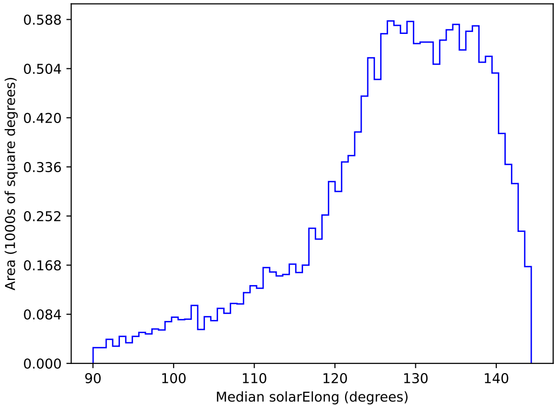
too_elab_r128_d2_griz_v3.4_10yrs WFD z band: Median solarElong
