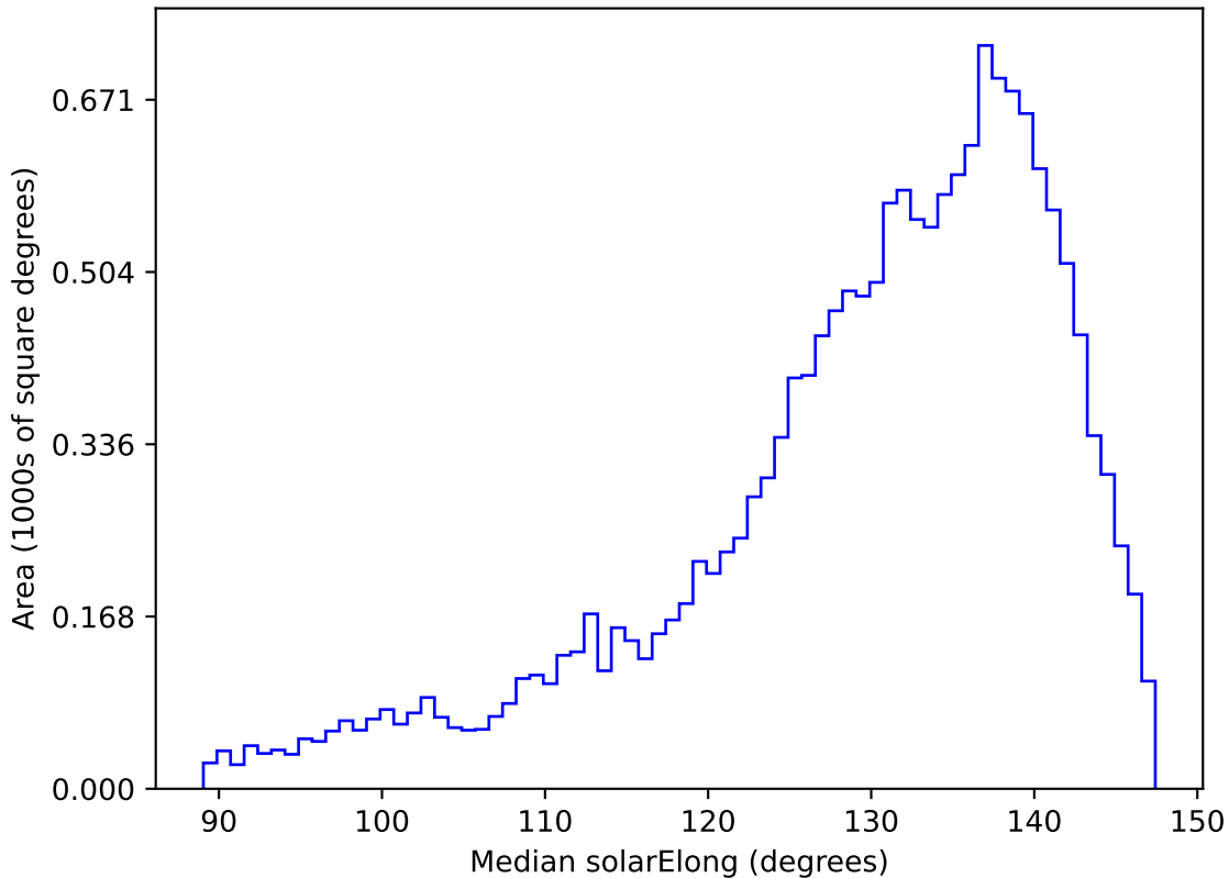
too_elab_r128_d2_griz_v3.4_10yrs WFD y band: Median solarElong
