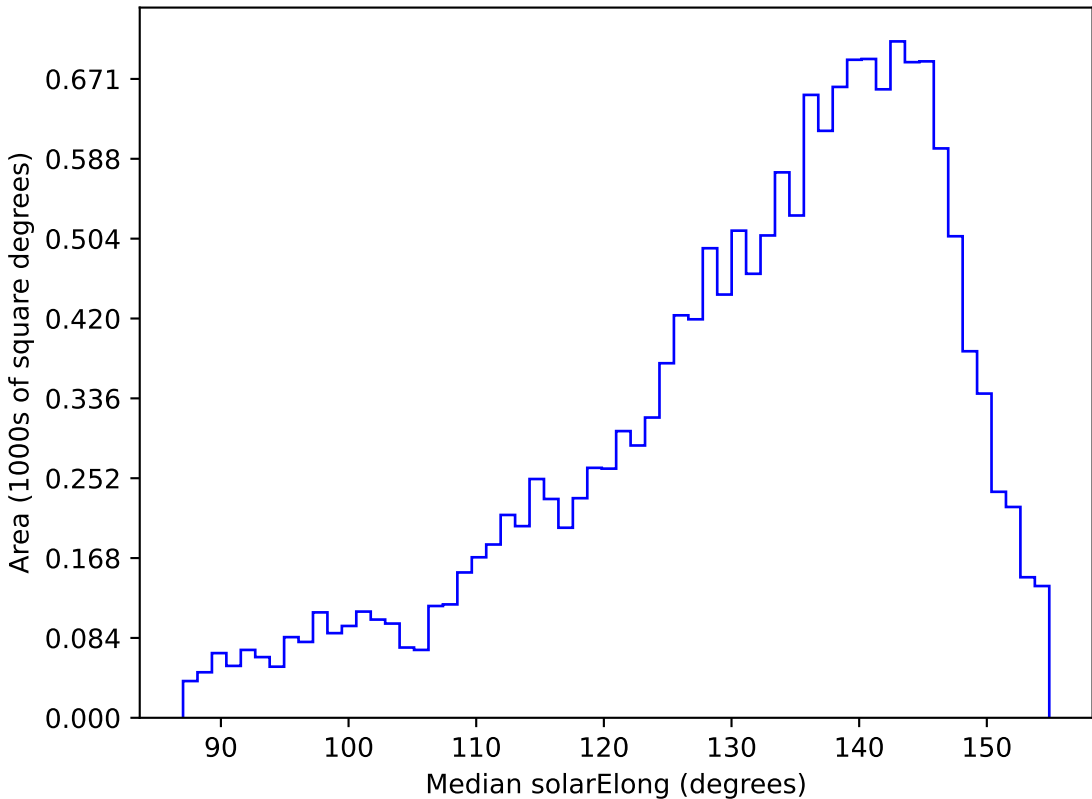
too_elab_r128_d2_griz_v3.4_10yrs WFD u band: Median solarElong
